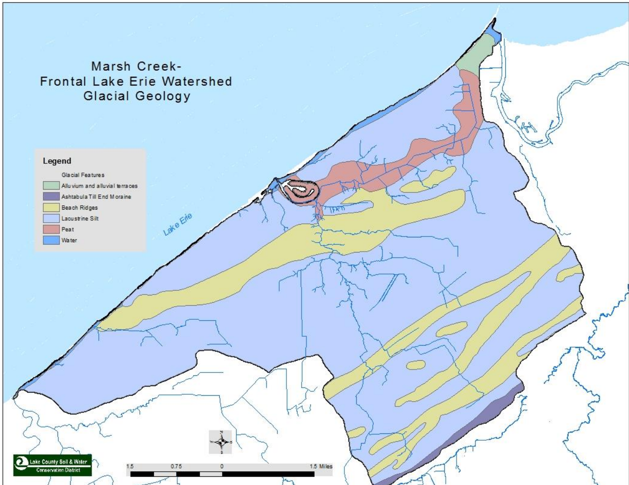
Figure 7: Glacial Geology
