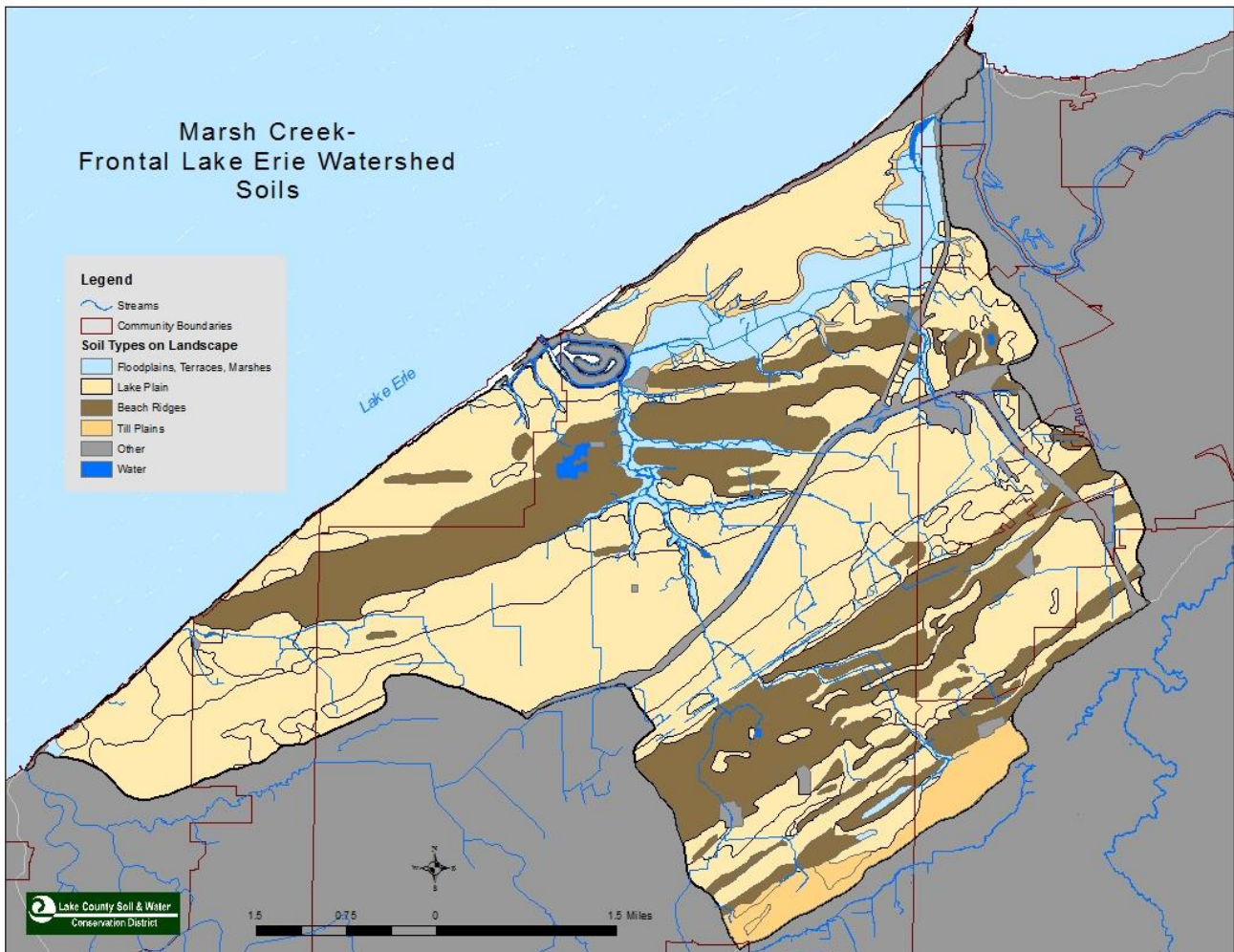
Figure 8: Soils
